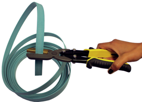
19HARDGUIDE CUTTER
